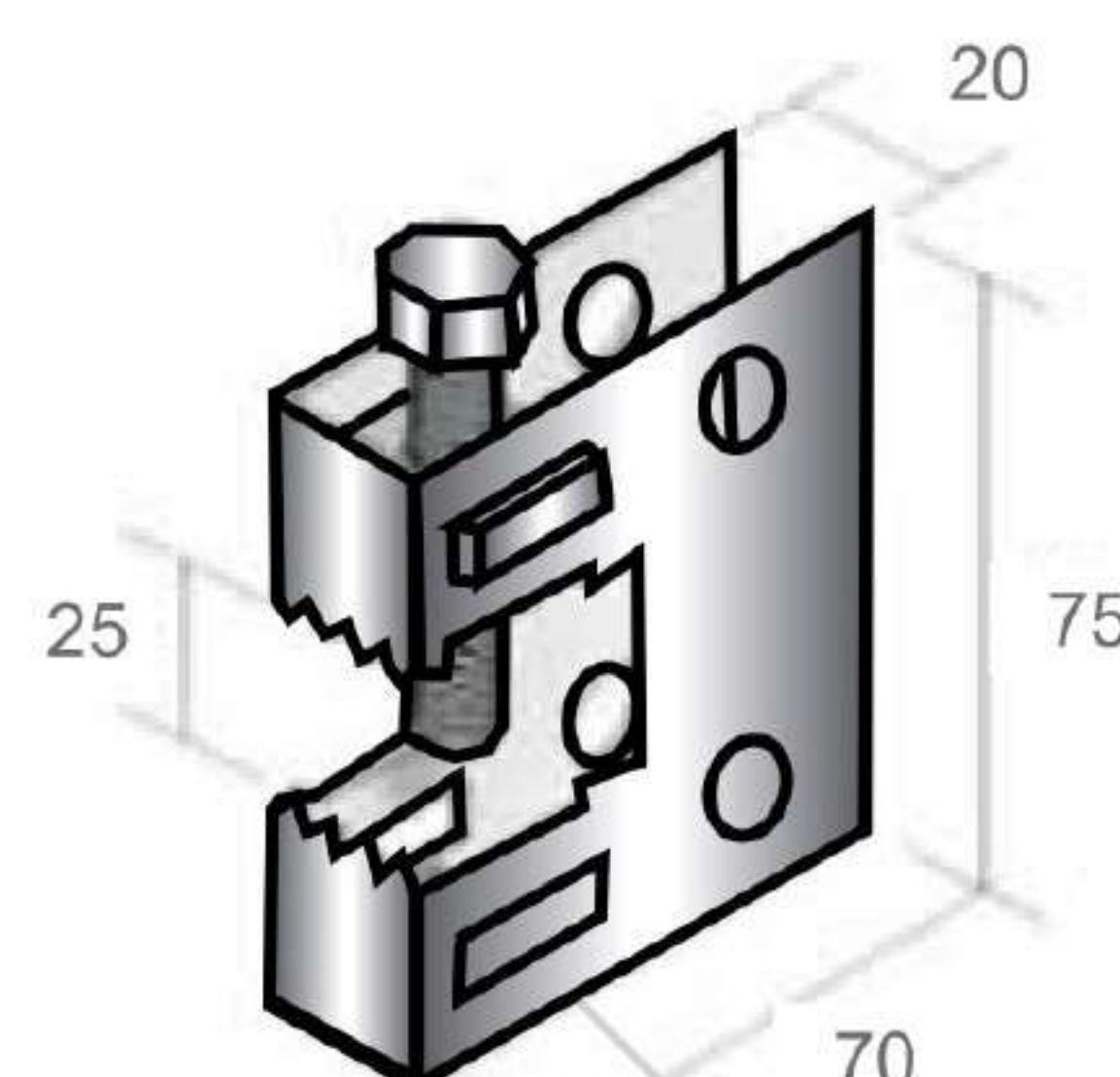
Grampo "C" ref: MG 820
