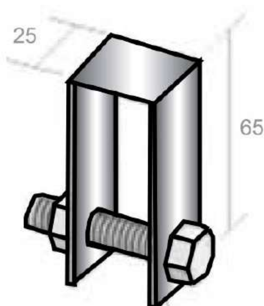
Balancim p/ Grampo "C" ref: MG 819
